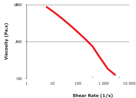
Shear-Viscosity @ 190 °C
